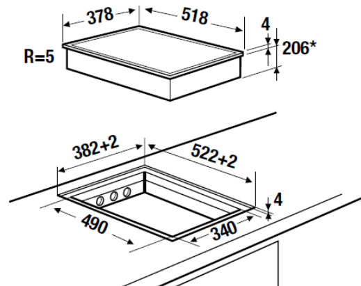
Flush installation
