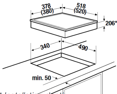
Top mount installation (with steel profiles)
